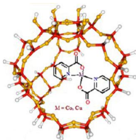
Figure 1.13 Structure of zeolite Y encapsulated metal picolinato complexes [80].
