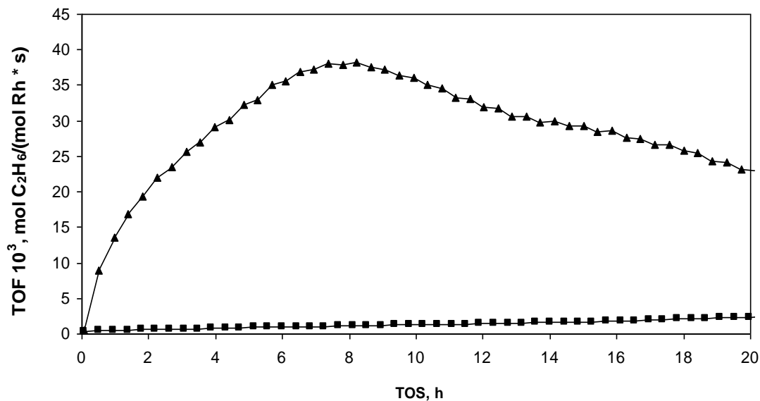
Figure 4.3 Rates (Turn Over Frequencies) of Ethane formation with Time on Stream (TOS) for Rh(CO) 2 /HY30 (▲), Rh(CO) 2 /γ-Al 2 O 3 (■) at 76 Torr of C 2 H 4 and 608 Torr of H 2 at ambient conditions.
