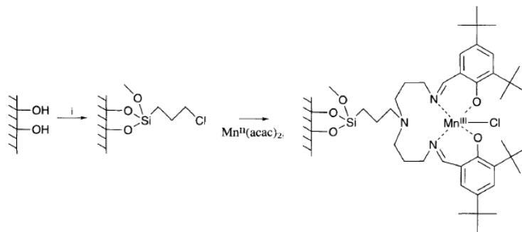
Figure 1.2 Manganese Schiff-base complexes anchored on MCM-41 [13].
