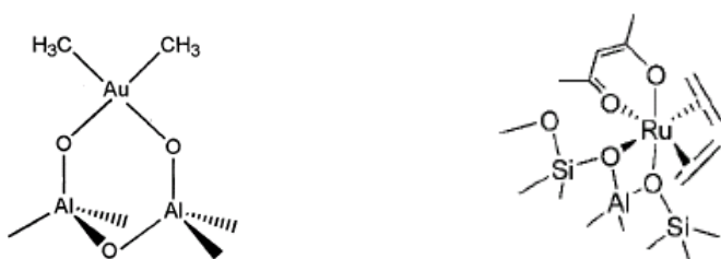
Figure 1.11 Proposed structures of HY zeolite-supported \text{Au}(\text{CH}_3)_2 and \text{Ru}(\text{C}_2\text{H}_4)_2(\text{acac}) complexes [59,60].
