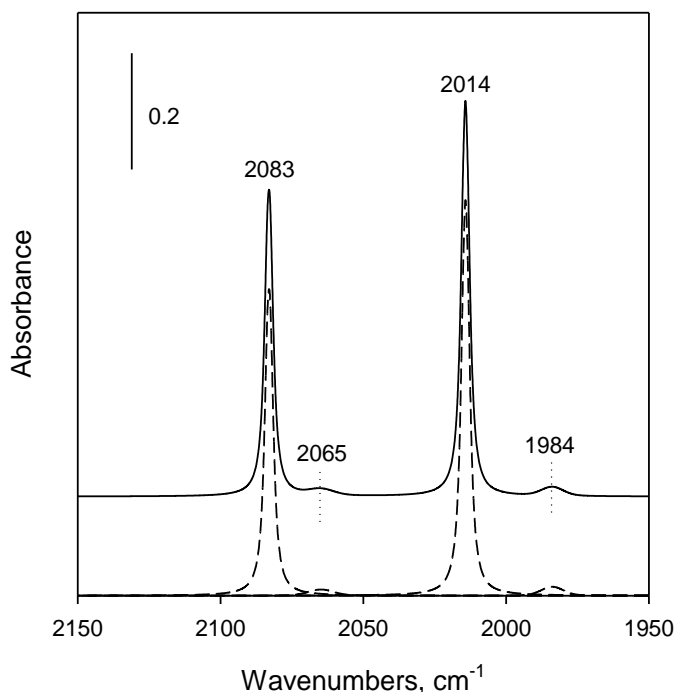
Figure 3.1 FTIR spectrum of \text{Rh}(\text{CO})_2(\text{acac}) in pentane (solid line) and deconvolution results (dashed line).
