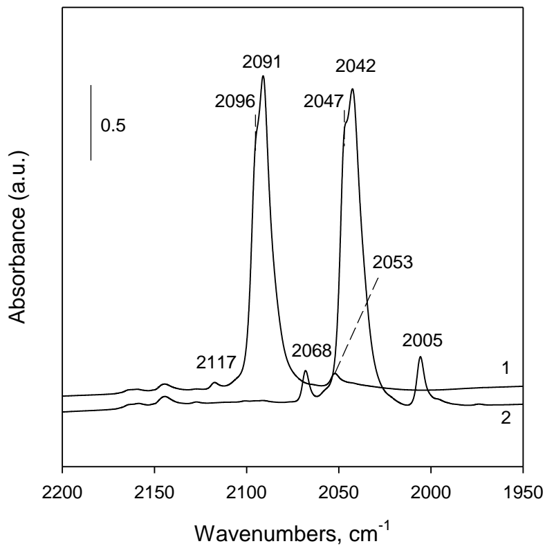
Figure 2.5 FTIR spectra of (1) \text{Rh}(\text{CO})(\text{C}_2\text{H}_4)/\text{HY30} and (2) \text{Rh}({}^{13}\text{CO})(\text{C}_2\text{H}_4)/\text{HY30} samples treated in \text{H}_2 at room temperature for 30 min.
