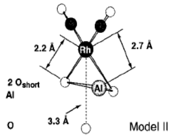
Figure 1.17 Simplified structural model for Y zeolite-supported \text{Rh}^+(\text{CO})_2 complexes developed from EXAFS data analysis [63].
