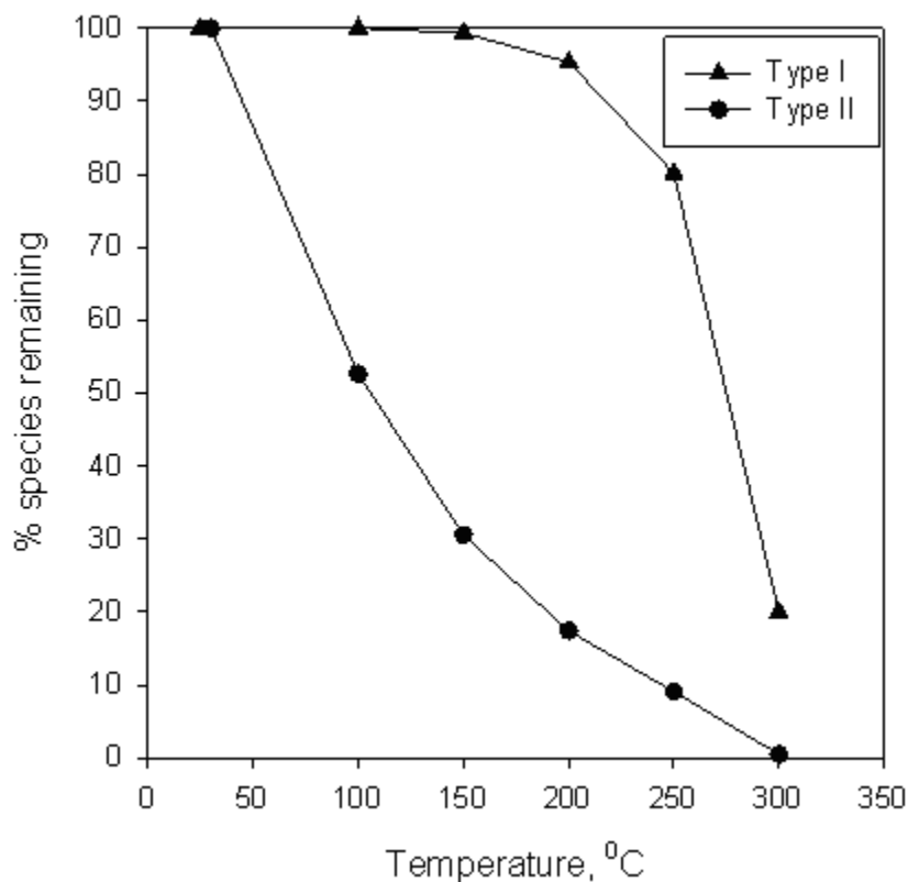
Figure 3.3 Percent of Rh dicarbonyls remaining on the surface of Rh(CO) 2 /HY2.6 during thermal treatments with He at different temperatures: (▲) type I ( \nu_{CO} at 2117/2053 cm -1 ) and (●) type II ( \nu_{CO} at 2110/2043 cm -1 ) species.
