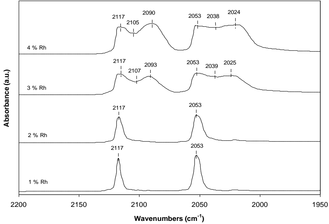
Figure 4.26 FTIR spectra in the \nu_{CO} region of Rh(CO)_2/HY30 at different Rh loading: 1, 2, 3, and 4 %wt.
